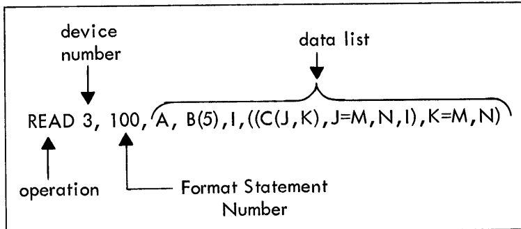
Figure 17 I/O Statement
