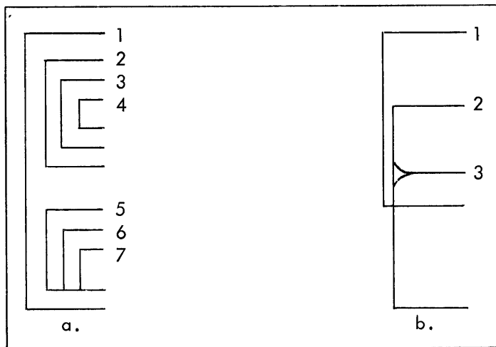
Figure 15 DO Loops
